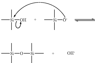
Figure 10: Nucleophilic Attach to Form Siloxane Bond
